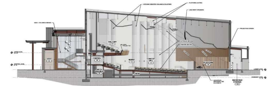
east-west building section
